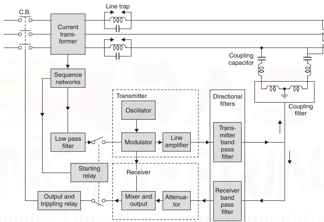
Fig. 14.59 Block diagram of equipment used in carrier phase comparison scheme.
