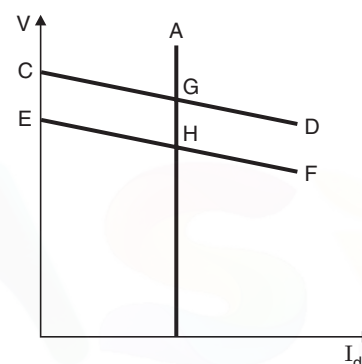
Fig. 5.17 Control characteristics.
