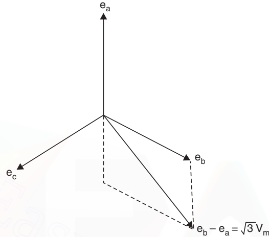
Fig. 5.6 Phasor diagram for evaluating limits of hatched area.
