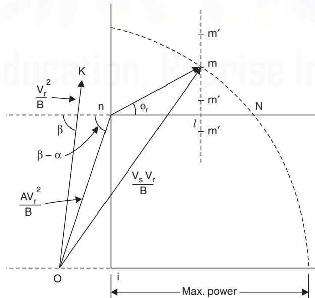
Fig. 22.2 Receiving end power circle diagram.
