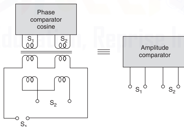
Fig. 14.68 Equivalence of amplitude comparator.
