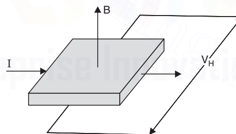
Fig. 14.83 Hall effect phase comparator.
