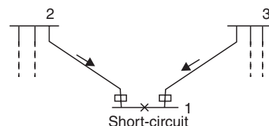
Fig. 13.26 A three-bus system with short-circuit at bus 1.
