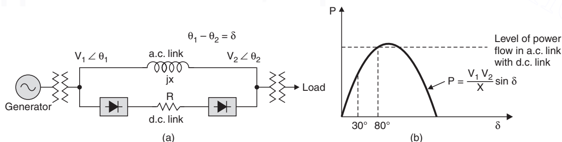
Fig. 5.23 (a) a.c. and d.c. connected in parallel (b) Power angle diagram for a.c. link.
