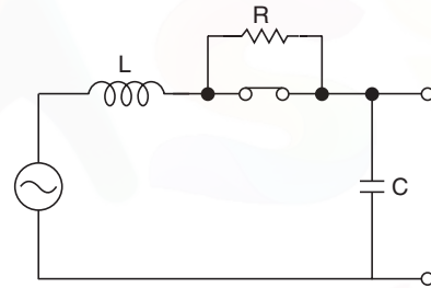
Fig. 15.3 Resistance switching.
