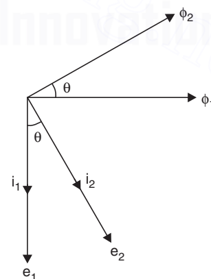
Fig. 14.3 Phasor diagram for an induction relay.
