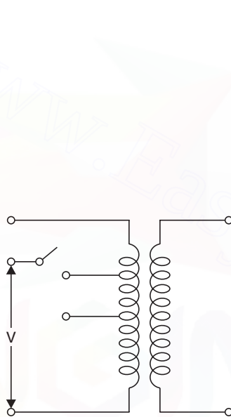
Fig. 10.7 Off-load tap changing transformer.
