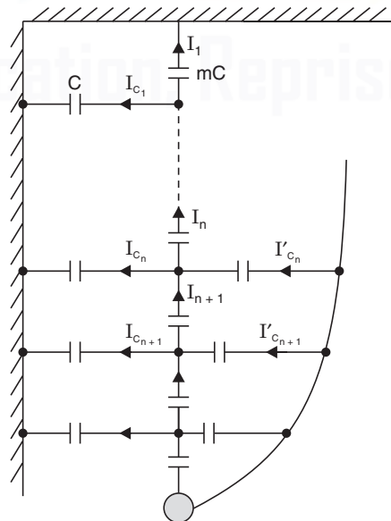
Fig. 8.6 Static shielding.
