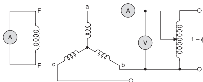
Fig. 13.3 Measurement of subtransient reactance of an alternator.
