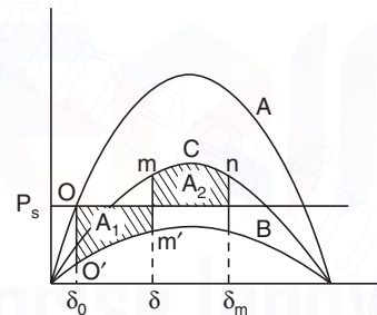
Fig. 17.12 Equal area criterion applied to system of Fig. 17.9 for a fault cleared at an angle \delta < \delta_0 .
