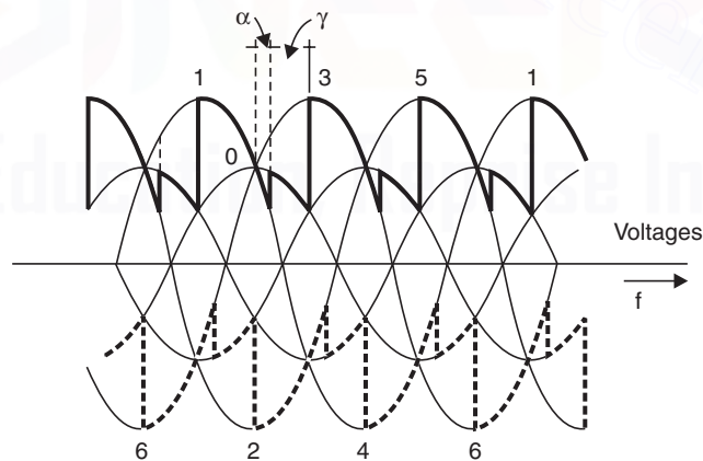
Fig. 5.5 Voltage waveform with grid control \alpha and overlap \gamma in case of bridge connection.
