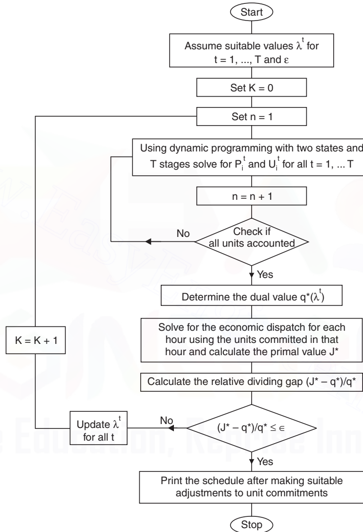
Fig. 24.2 Flowchart for Lagrange relaxation method for UC.
