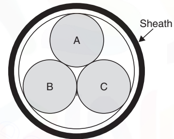
Fig. 9.25 Breakdown of a 3-phase belted cable.
