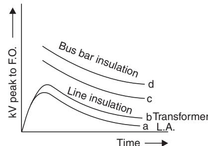
Fig. 16.3 Volt-time curves
