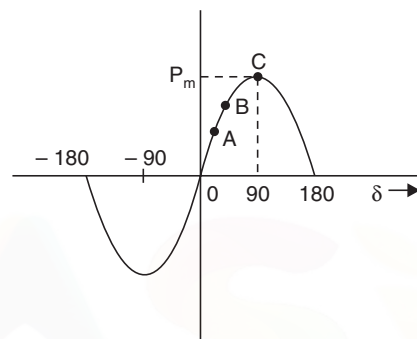
Fig. 17.3 Power angle curve.
