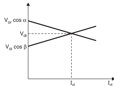
Fig. 5.14 Operation diagram.
