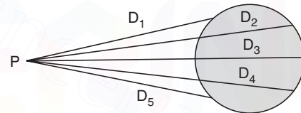
Fig. 2.10 Distances from an external point to five points on a circle.
