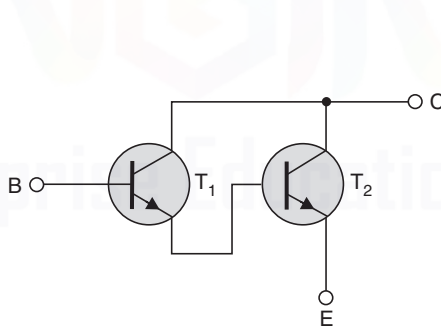
Fig. 14.93 Darlington circuit.
