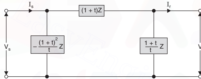
Fig. 18.4 Equivalent circuit of a transformer for nodal admittance matrix.
