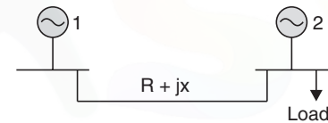
Fig. 19.3 Two identical generators connected through a transmission link.
