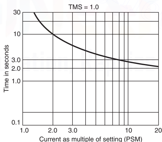
Fig. 14.7 Standard 2.2 sec IDMT curve.
