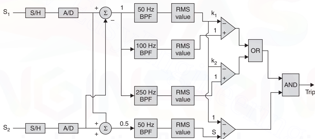
Fig. 14.129 Percentage differential relay.
