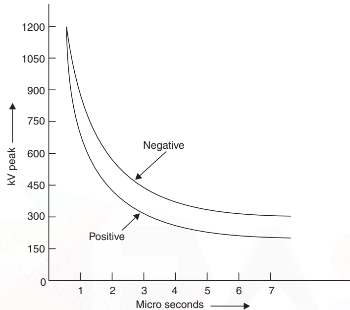
Fig. 16.5 Volt-time curves of gaps for positive and negative polarity.
