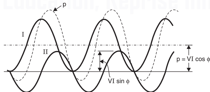
Fig. 1.2 Active, reactive and total power in a single phase circuit.
