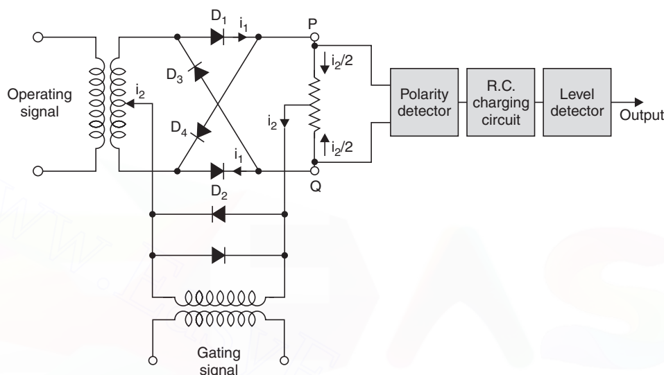
Fig. 14.82 Basic circuit of an integrating phase comparator using rectifier bridge AND gate.
