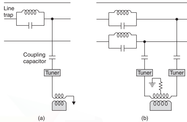
Fig. 19.9 Coupling circuits (a) centre-phase to ground and (b) adjacent phase to phase.
