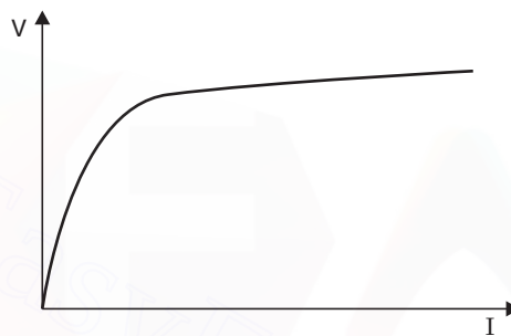
Fig. 21.21 Characteristic of a saturated reactor compensator.
