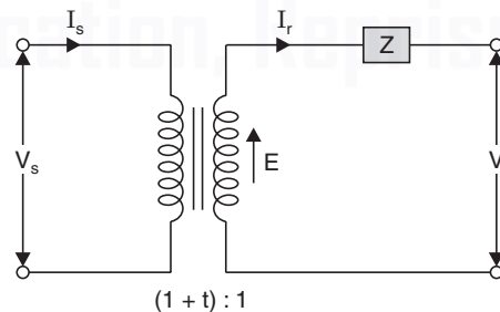
Fig. 18.3 Elementary transformer connection
