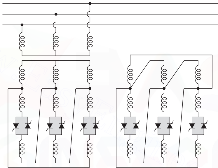
Fig. 21.16 12-pulse TCR arrangement with double secondary transformer.
